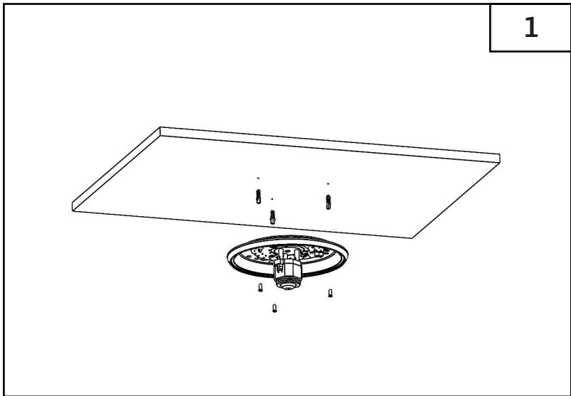
1.1 Ölçülere uygun bağlantı delikleri delinir.Ürün kasası civatalarla tavana monte edilir. 1.1 Connection holes are drilled in accordance with the dimensions. The product casing is mounted to the ceiling with bolts.
