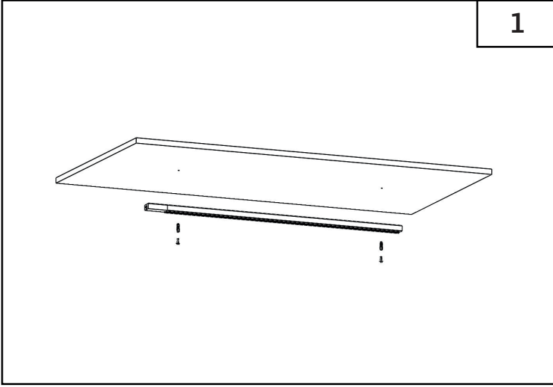
1.2 Ray, montaj deliklerinden tavana monte edilir. 1.2 The rail is mounted to the ceiling through the mounting holes.
